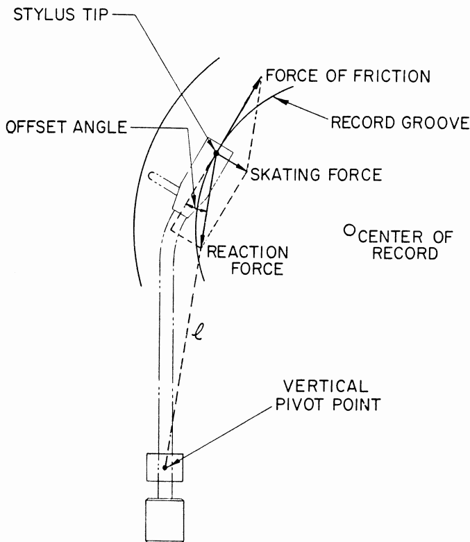
Fig. 1. Position of the arm on the record.
