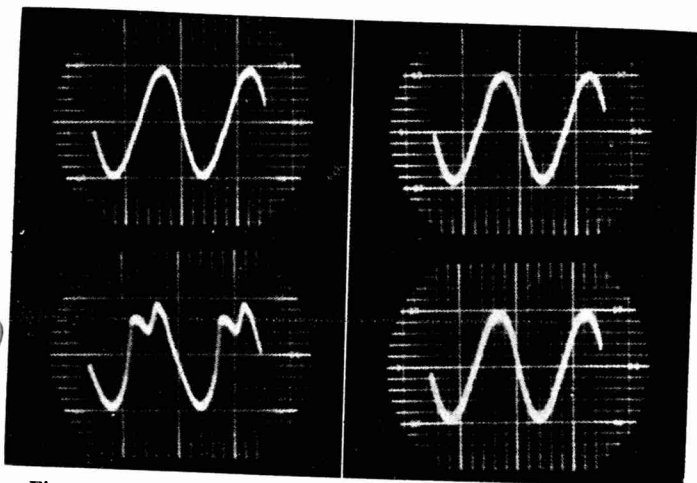
Fig. 5. Application of anti-skating to the tracing of a high level stereo groove. a. without, and b. with anti-skating provisions.
